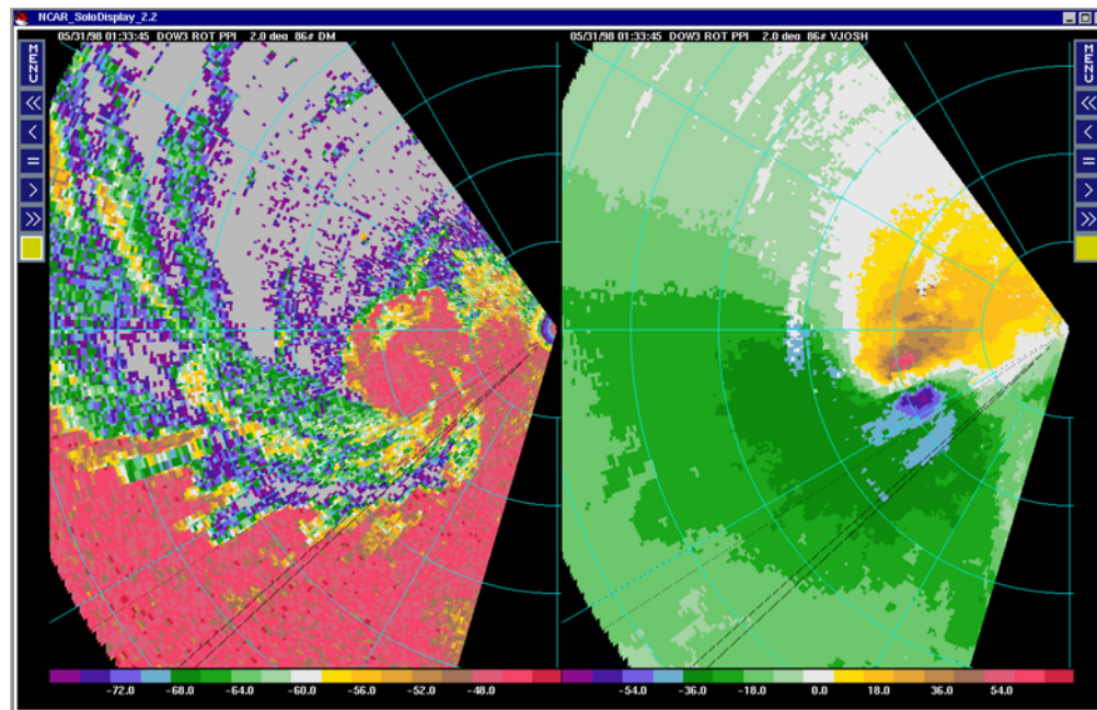
Reflectivity (Left) and Doppler Velocity (Right) in strong tornado that destroyed much of Spencer, South Dakota on 30 May, 1998.
