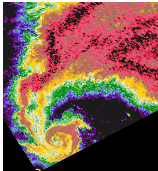
Reflectivity during tornadogenesis near Rolla, Kansas on 31 May, 1996.
